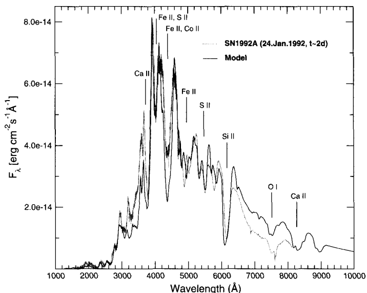
Fig. 1. Synthetic spectrum for a SN Ia around maximum light based on the W7 explosion model with homogenized composition. For comparison, the observed spectrum of SN1992A is also plotted.
