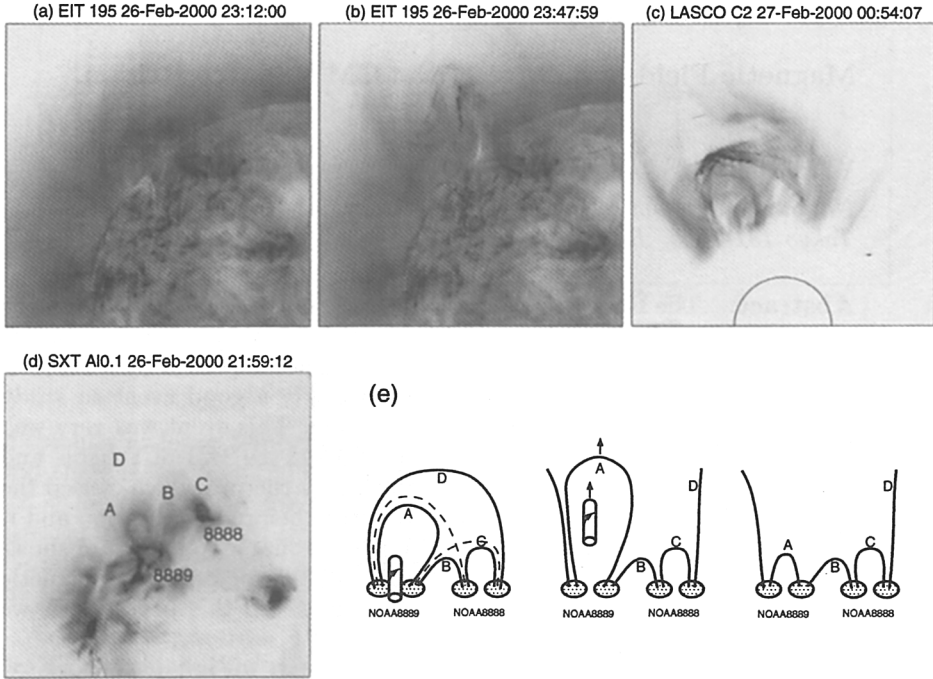
Figure 1. CME and filament eruption observed with (a-b) the EIT and (c) the LASCO of SOHO. (d) The coronal loop structure observed with the SXT of Yohkoh just before the eruption. All images are shown in negatives. (e) Schematic drawing of the filament and the coronal loops in the CME source region before, during, and after the eruption.
