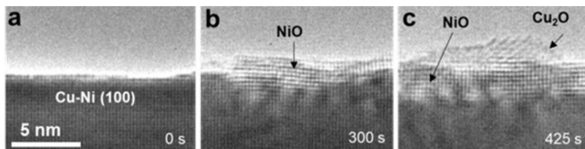
Figure 2. Figure 2. In situ observation of oxide growth on Cu-Ni(100) alloy (10 at.% Ni) at 350 °C under 0.1 Pa O 2 . (a) Clean alloy surface in vacuum. (b) Nucleation and growth of epitaxial NiO. (c) Secondary nucleation and growth of Cu 2 O.
