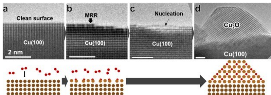
Figure 1. Figure 1. In situ ETEM observation of initial oxidation processes on pure Cu(100) surfaces at 350 °C under O 2 . (a) Clean Cu(100) surface in vacuum. (b) Missing Row Reconstruction (MRR) on stepped Cu(100) surface under 0.1 Pa O 2 . (c) Cu 2 O nucleation on Cu(100) surface under 0.3 Pa O 2 . (d) Cu 2 O island growth under 0.3 Pa O 2 . Scale bars: 2 nm.
