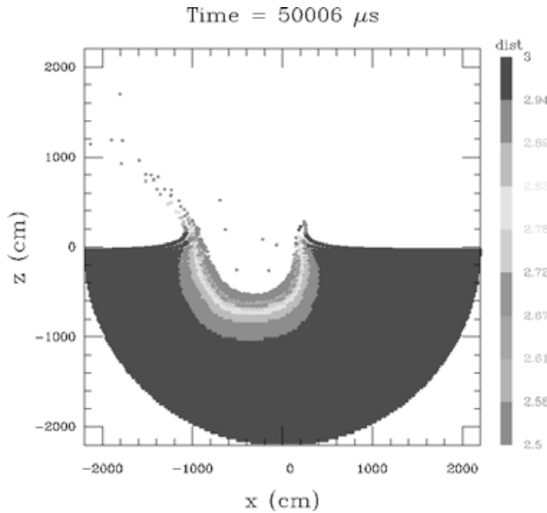
Figure 2. A measure of the compaction is provided by the actual value of the distention \alpha . The initial distention of \alpha_0=3 is decreased to \alpha=1 in a small zone around the crater. With increasing distance from the crater, distention increases until \alpha = \alpha_0
