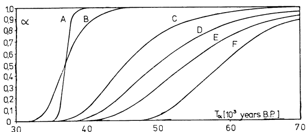
Fig 1. Probability \alpha of the verity of the relation T < T_\alpha as a function of T_\alpha for some values of N'/M and \sigma/M M: modern counting rate, N' and \sigma : measured sample counting rate and measuring error. N'/M and \sigma/M are equal, respectively, for the curves A: 0.01, 0.001; B: 0.01, 0.003; C: 0.003, 0.003; D: 0, 0.003; E: 0, 0.001; F: -0.003, 0.003.
