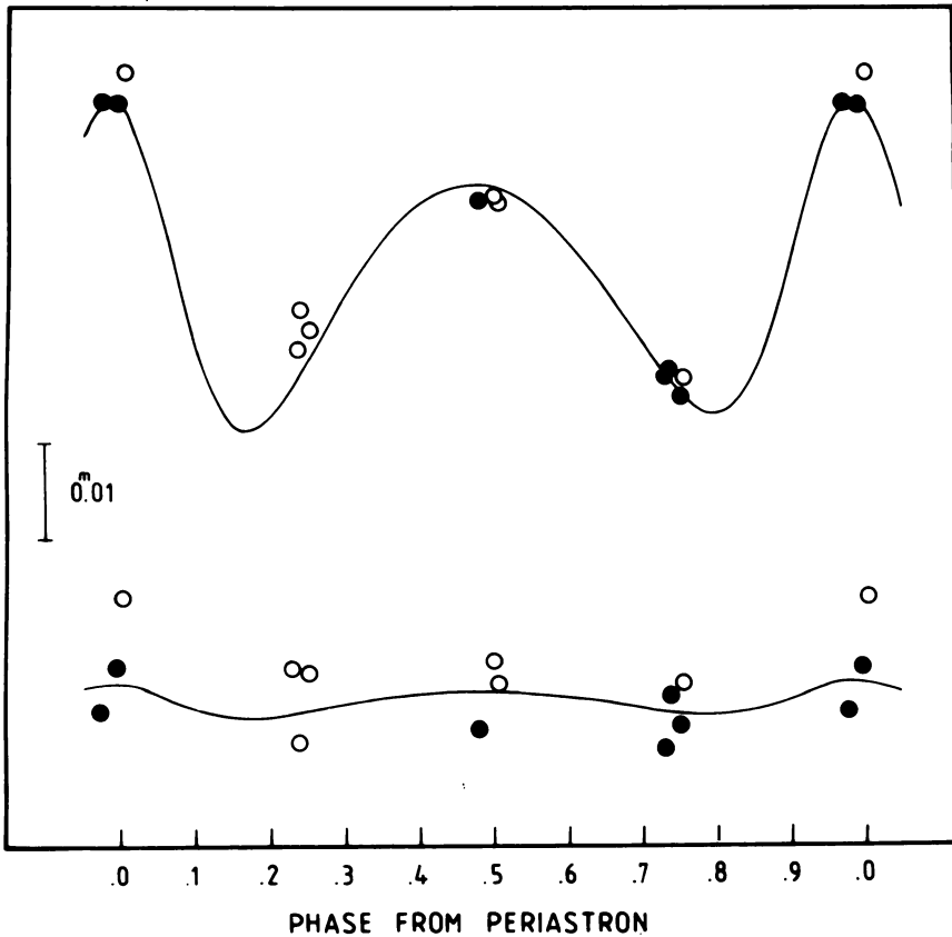
Figure 1. The nightly differential \gamma magnitudes (top) and c_i indices (bottom), Spica minus \theta Vir, plotted as a function of the orbital phase. Open circles denote single observations or means of not more than three observations, whereas filled circles denote means of eight or more observations. The solid lines represent the computed ellipsoidal light and colour index variations, referred to in Section 3.
