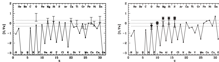
Figure 1. Abundance pattern of our 1000M_{\odot} star model and observational data. (left panel) EMP stars (Cayrel et al. (2004)). (right panel) ICM (bars, Baumgartner, et al. (2005)), and hot gas in M82 (pentagons, Origlia et al. (2004)).
