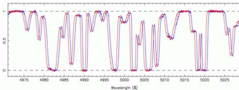
Figure 1. Simulated spectra of the Ly \alpha forest of a QSO taken with a time interval of 10^7 yrs. The shift due to the cosmic acceleration is clearly visible.
