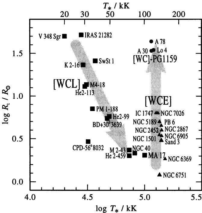
Figure 1. Central stars of Wolf-Rayet type in the R_t - T_* -diagram. [WCL], [WCE] and [WC]-PG 1159 subtypes are represented by squares, triangles and circles, respectively. The shaded arrows suggest a possible evolutionary connection.
