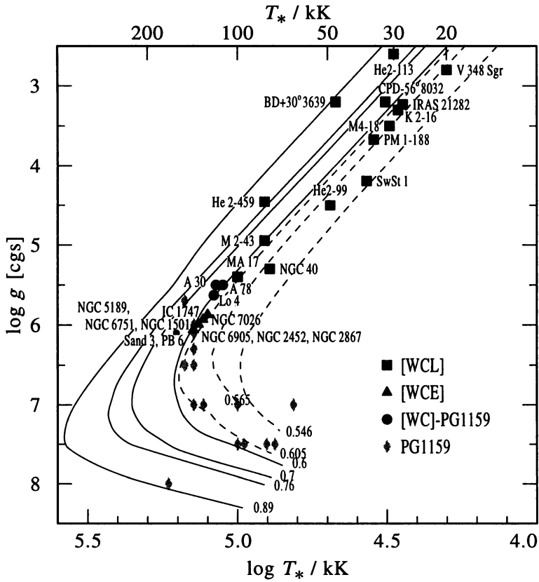
Figure 2. Central stars of Wolf-Rayet type in the \log g - \log T_* -diagram. [WCL], [WCE] and [WC]-PG 1159 subtypes are represented by squares, triangles and circles, respectively. Shaded diamonds indicate “normal” PG 1159 stars without strong mass-loss (after Dreizler et al. 1995). The tracks for post-AGB evolution taken from Schönberner (1983) or Wood & Faulkner (1986) (labels: mass in M_\odot ) and are only shown for rough comparison; they are not really adequate for the considered objects, as they predict normal surface abundances.
