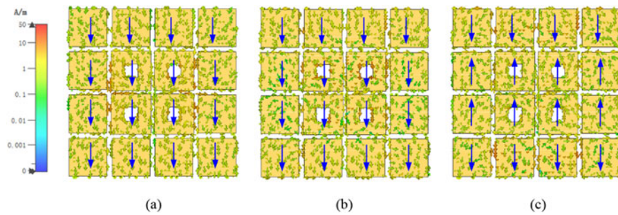
Figure 6. Current distributions of antenna: (a) at 5.0 GHz, (b) at 6.0 GHz, and (c) at 7.0 GHz.
