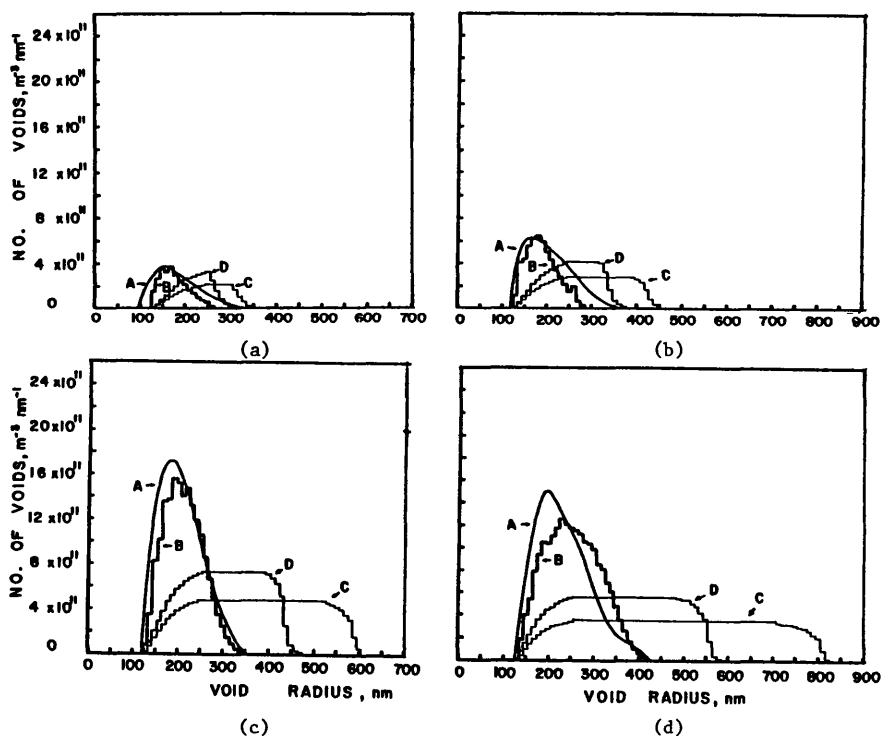
FIG. 5. Void size distribution curves for Cu crept at 405°C under a stress of 27.6 MPa for (a) 1.1 \times 10^4 s, (b) 2.2 \times 10^4 s, (c) 4.3 \times 10^4 s, (d) 7.7 \times 10^4 s. Smooth curves (A) are obtained from the SANS measurements. The other curves are calculated on the basis of void growth models based on grain boundary vacancy diffusion (B), and diffusion coupled with matrix plasticity with (D) and without (C) surface energy forces taken into account [13].
