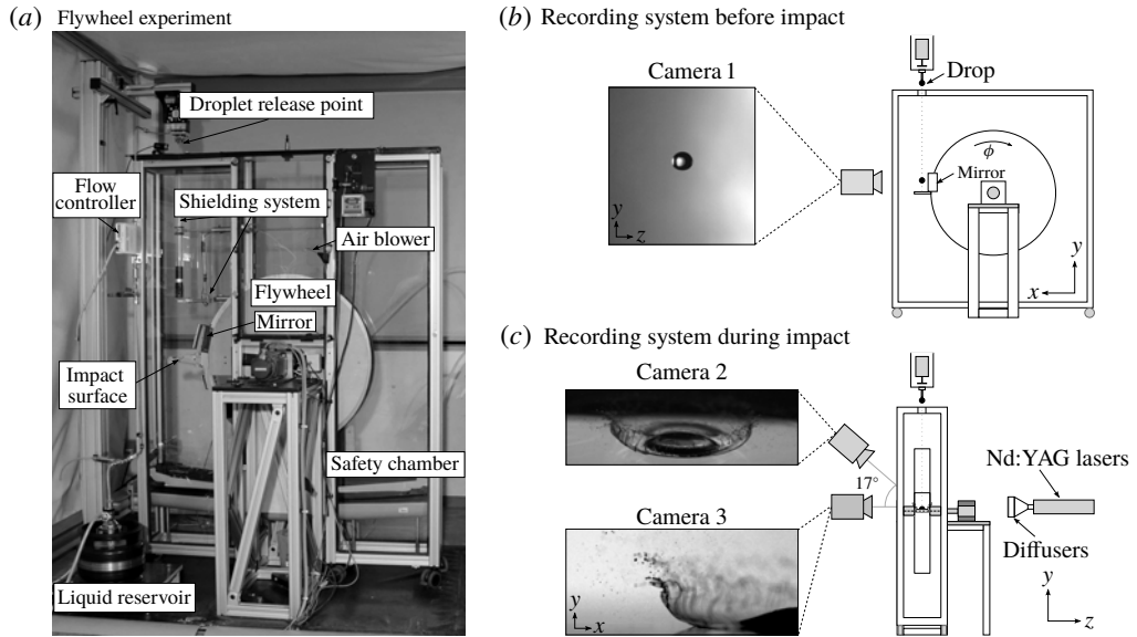
FIGURE 4. Experimental method. Panel (a) shows a picture of the flywheel experiment indicating its principal components. Panels (b,c) illustrate the shadowgraph set-up used to capture the droplets before and during impact. The images show an example of the same ethanol drop D = 2.4 mm impacting the surface at U = 6.3 m s -1 ( We = 3300 , Re = 9500 ).
