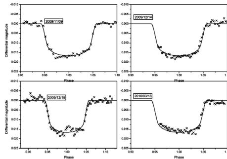
Figure 1. Binned light curves of WASP-12b and relative fitting.
