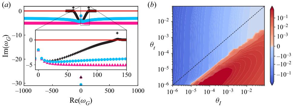
Figure 5. (a) Comparison of the eigenspectra of the case with \theta_t \ll 1 and \theta_I \ll 1 (+), the case with \theta_t \ll 1 but \theta_I = 0 (●, blue), and the case with \theta_I = 0 and \theta_t = 0 (▲, pink). The dimensionless parameters are taken as per case C3 in table 5. (b) Contour plot of \text{Im}(\omega_G) of the least stable mode as a function of \theta_I and \theta_t , with \widehat{Re} and \beta taken from case C3 in table 5. The dashed line marks \theta_I = \theta_t .
