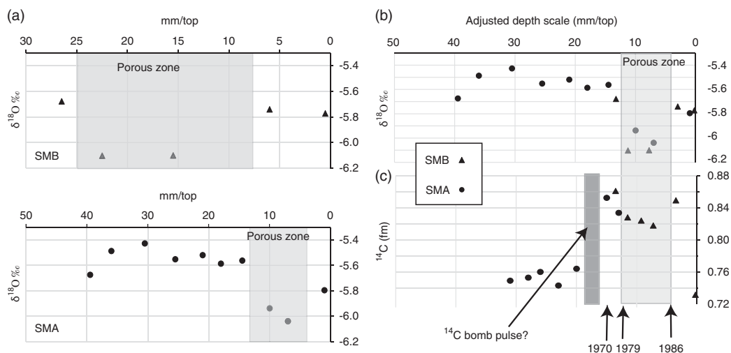
Figure 2 δ 18 O measured on SM-A and SM-B with proper depth scale (a) and adjusted depth scale (b); 14 C values according to adjusted depth scale.
