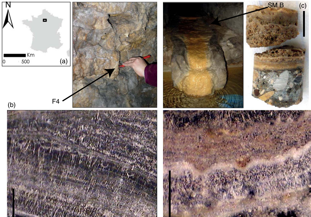
Figure 1 a) Location b) F4 sample from Versailles underground gallery before sampling (top), and picture of the thin section showing laminae (with the black vertical bar representing 2 mm); c) Saint Martin spring and the CaCO 3 crust sampled (arrow), SM B core (with black bar representing 20 mm) and picture of thin section within the laminated level (with the black vertical bar representing 2 mm).
