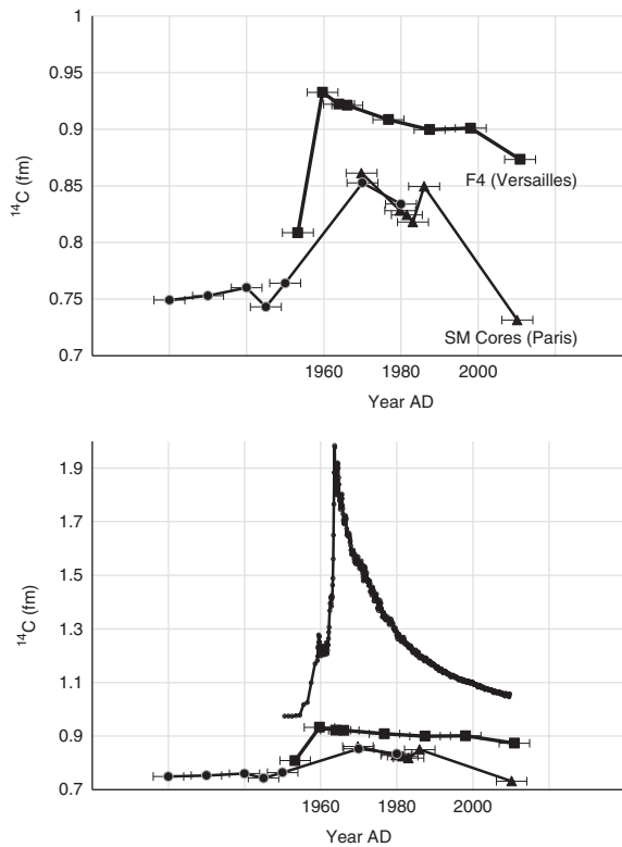
Figure 4 Top: Comparison between Saint Martin and Versailles 14 C records. Bottom: Comparison between atmospheric (Hua et al. 2013) and speleothem 14 C records.
