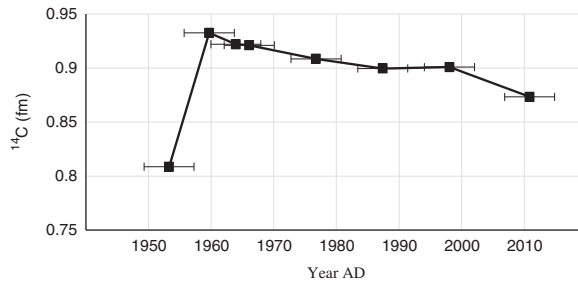
Figure 3 14 C trend vs laminae counting derived age for F4 sample (Versailles gallery)
