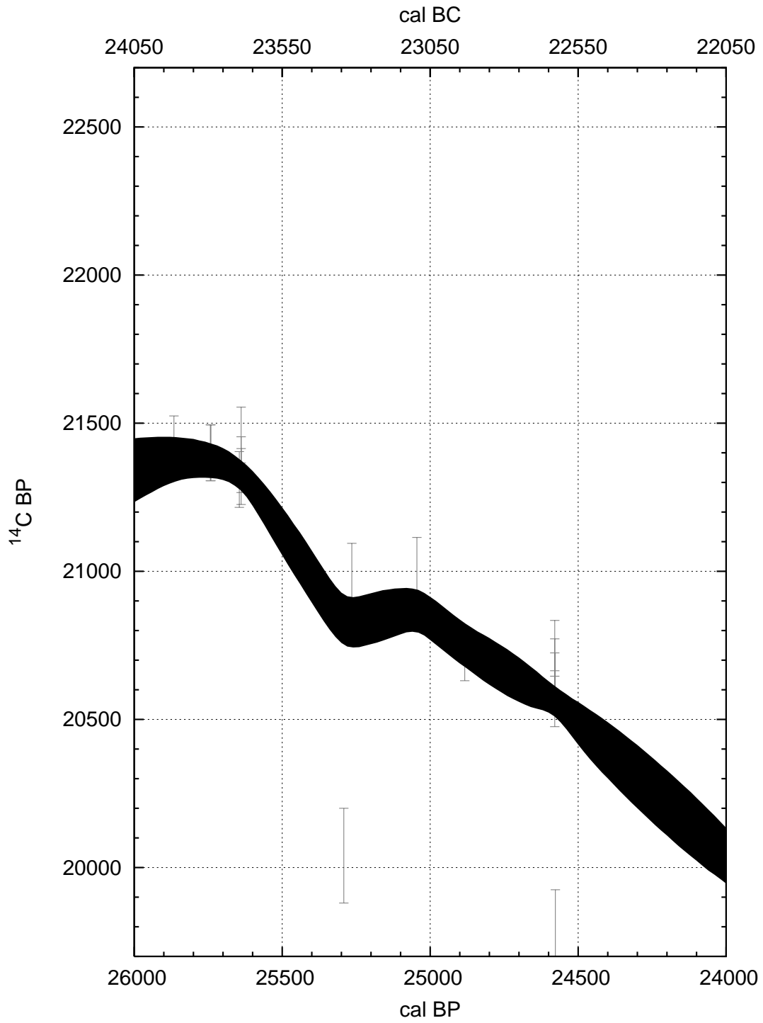
Figure A1 The IntCal04 terrestrial calibration curve (1-standard deviation envelope) and data with 1-standard deviation error bars in ^{14}\text{C} increased by the laboratory error multipliers described in the text. The uncertainty in the calendar ages is not shown, but is taken into account in the random walk model.
