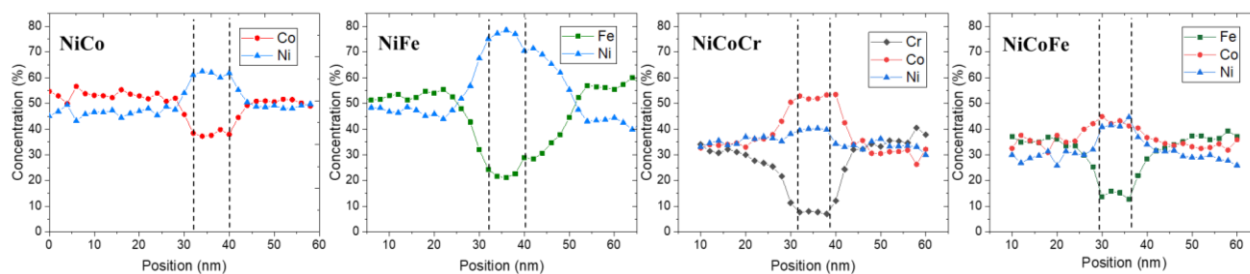
Figure 2. One-dimensional elemental concentration profiles across He bubbles in Ni-based CSAs. Position of He bubble is marked by two dashed vertical lines in each profile.
