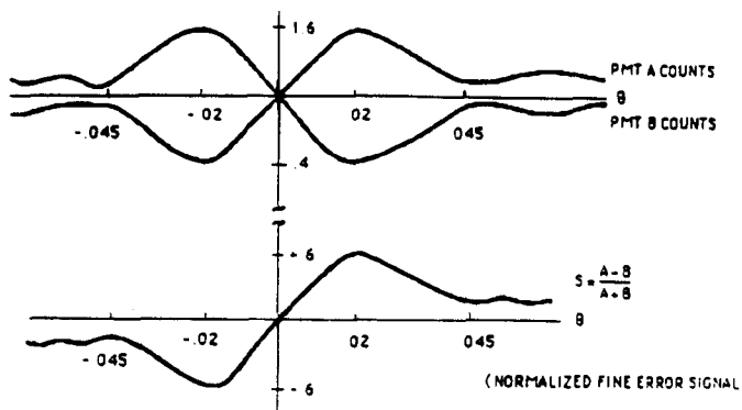
CONSTRUCTION OF A HYPOTHETICAL S-CURVE
