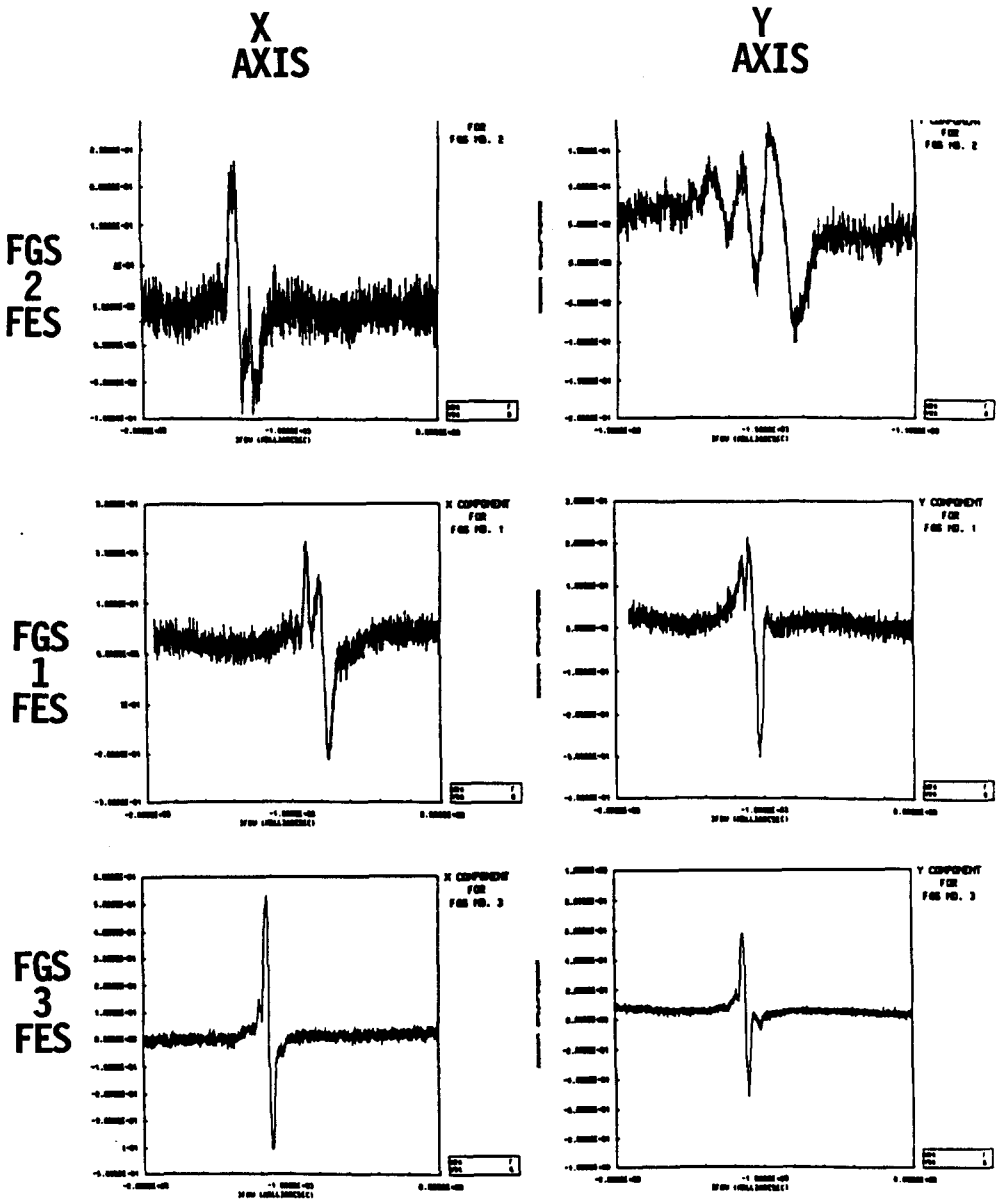
X AND Y TRANSFER FUNCTIONS OBSERVED IN FGSs 2, 1, AND 3 (top to bottom) Normalized Fine Error Signal vs Positional Offset
