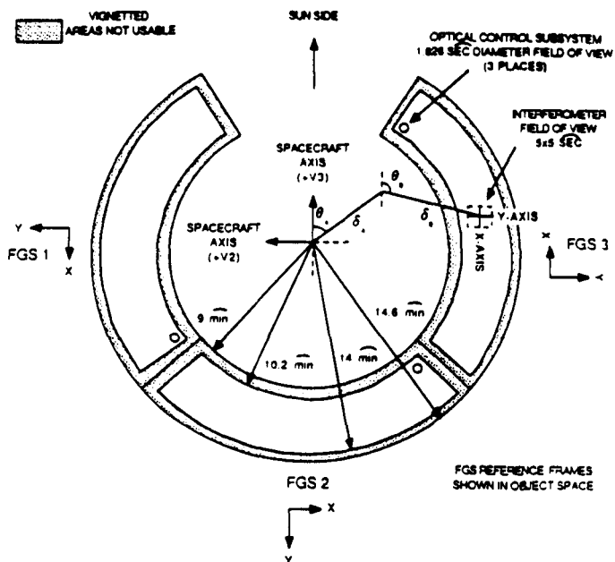
FGS FIELD OF VIEW PROJECTED ONTO THE CELESTIAL SPHERE
