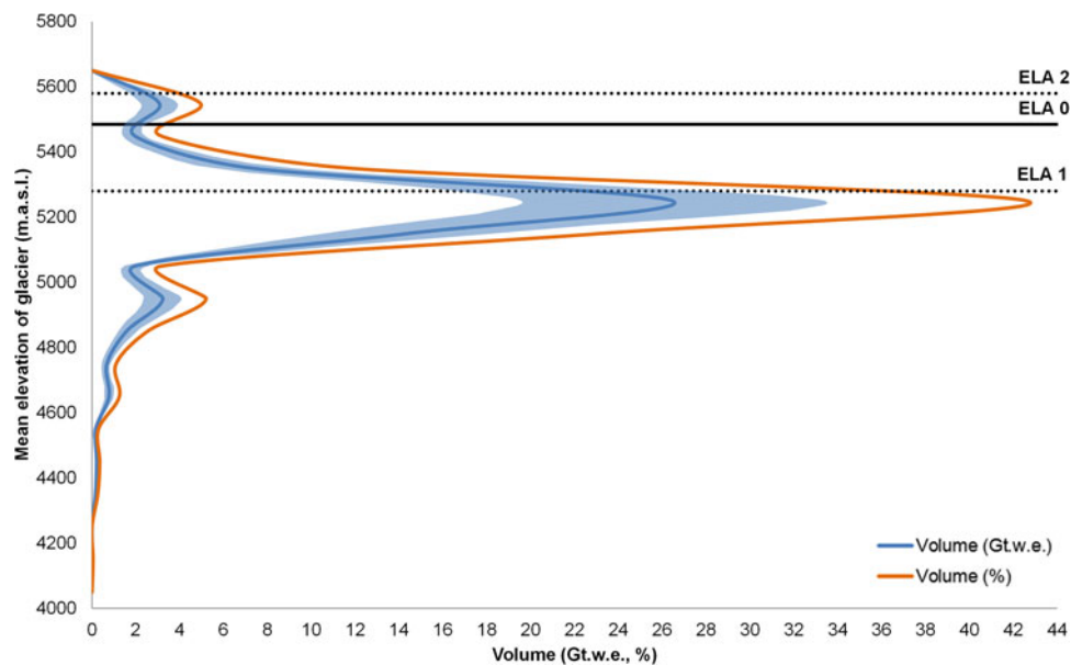
Fig. 7. Hypsometric distribution of volume with respect to the mean glacier elevation in the Chandra basin. Blue line represents volume in Gt w.e., with shaded area as uncertainty. Orange line represents fractional (%) volume stored at each elevation band. ELA0 is the mean ELA of the basin from 1984 to 2012. ELA1 and ELA2 are the mean ELAs of the decades 1985–95 and 1995–2005, respectively.
