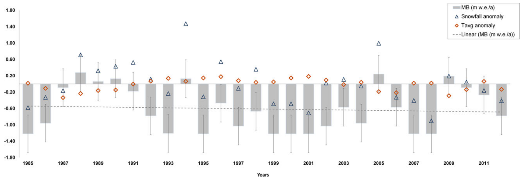
Fig. 4. Modelled annual specific mass-balance estimates of Chandra basin from 1984 to 2012. Bar plot represents area-weighted mean mass balance ( \text{m w.e. a}^{-1} ) for the basin. The uncertainty in model-derived mass balance is shown as vertical lines on the boxes, i.e. \pm 0.46 \text{ m w.e.} The grey dashed line is the linear regression line for the mass balance and indicates a mass-balance trend of -0.11 \text{ m w.e. a}^{-1} decade ^{-1} . Orange diamonds represent normalised (by mean) anomaly in summer temperature, and blue triangles represent normalised anomaly in winter snowfall. It is found that almost all the positive mass-balance years are accompanied by positive anomaly in snowfall and negative anomaly in temperature.
