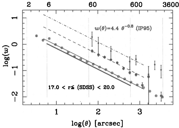
Figure 1. Angular Correlation Function of galaxies, pairs and triplets for 17 \leq r^* \leq 20 . The dark solid line is the IP95 (Infante & Pritchett 1995) w(\theta) result with \delta = -0.8 . The thin solid line is the model for galaxies with ( r_o = 4.5 h^{-1} Mpc). The dashed line is a model for pairs with ( r_o = 8.0 h^{-1} Mpc). The dashed dotted line is a model for triplets with a large correlation length ( r_o = 14.5 h^{-1} Mpc). All models are for \epsilon = 0.8 .
