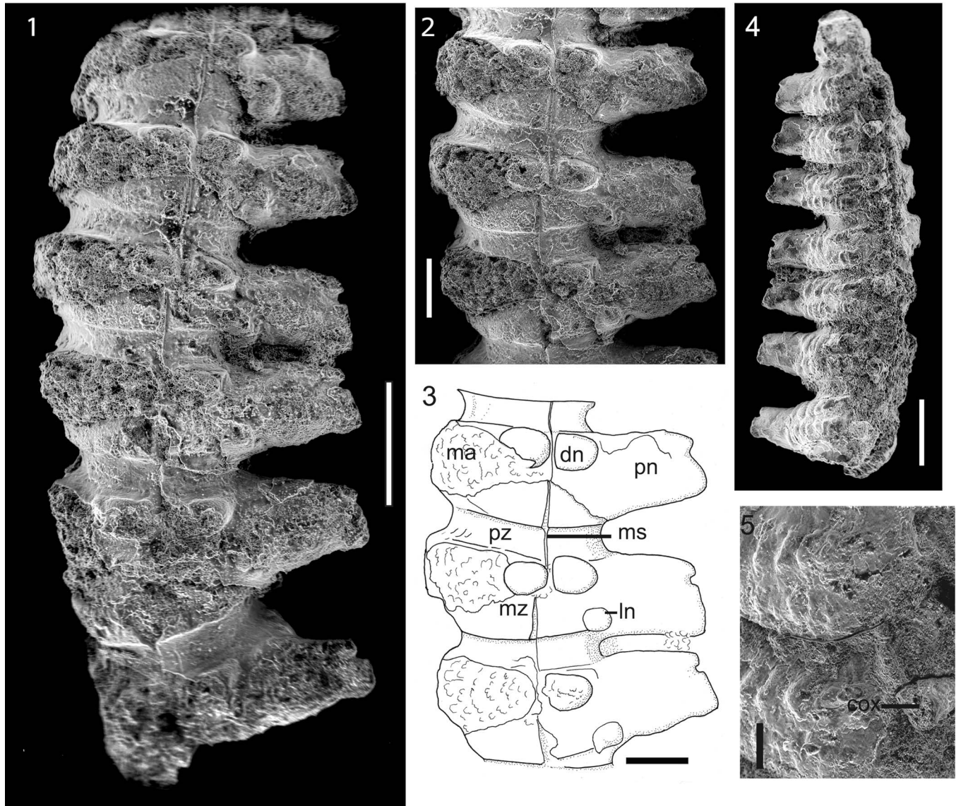
Figure 2. Oklahomasoma richardsspurense n. gen. n. sp., OU 44526, SEM microphotographs except for drawing. (1) Dorsal view; (2) close-up of dorsum; (3) interpretive drawing of (2) identifying features noted in text; (4) ventral view, slightly tilted to better see left side; (5) close-up of ventral side of two segments and one coxal segment. dn = dorsal node; cox = coxa; ln = lateral node; ma = mineralized area where cuticle is missing; ms = mid-dorsal suture; mz = metazonite; pn = paranota; pz = prozonite. (1, 4) Scale bars = 1 mm; (2, 3) scale bars = 500 \mu ; (5) scale bar = 200 \mu .
