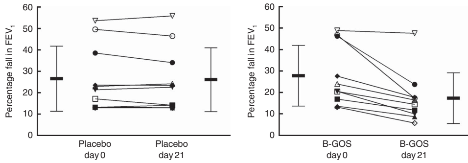
Fig. 3. The individual data and mean values and standard deviations for the peak fall in forced expiratory volume in 1 s ( FEV_1 ) after eupnic voluntary hyperpnoea in hyperpnoea-induced bronchoconstriction participants only. Individual participants are represented by the same symbols in both the placebo and B-GOS figures. B-GOS, Bimuno-galactooligosaccharides.
