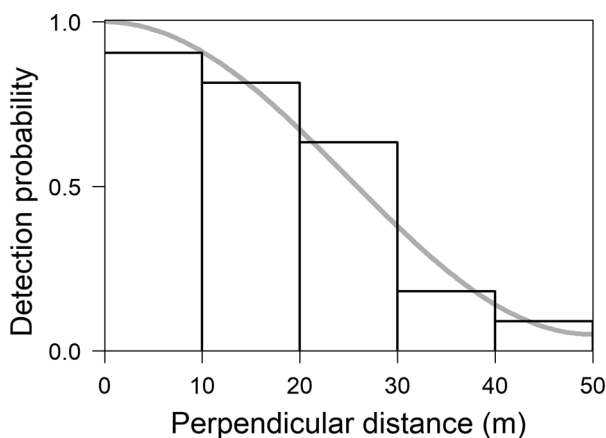
FIG. 2 Distribution of perpendicular distances of observations of M. marcai on transects in the Marmelos–Ariupanã interfluvium (Fig. 1). The trend line indicates the best detection function fitted to the distance classes.
