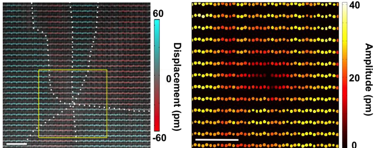
Figure 2. (a) STEM image of Zr-doped \text{ErMnO}_3 with a color overlay corresponding to the Er displacement, with turquoise indicating a positive polarization and red indicating negative. A vortex center is observed where 6 domains meet. (b) Amplitude of the ferroelectric displacement of the Er atoms shown in the yellow box in (a), showing vanishing amplitudes near the vortex center. Scale: 2nm.
