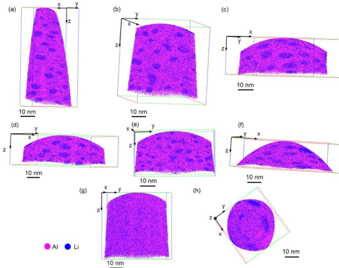
Figure 1. Comparison of the morphology of the \delta' precipitates under illumination of the laser pulses at various values of energy E measured for different samples: (a) 10, (b) 30, (c) 40, (d) 50, (e) 60, (f) 80 and (g, h) 100 pJ.
