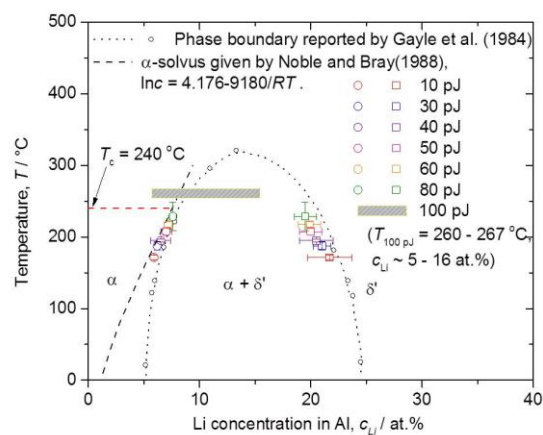
Figure 2. Comparison of the experimental Li concentrations and the estimated temperatures with an Al-Li phase diagram adapted from Ref [2]. The data obtained at E = 10 - 80 pJ agree with the miscibility gap, at well below the T_c . At 100 pJ, the tip temperature is estimated to be in the range of solvus temperature of \delta' precipitates.
