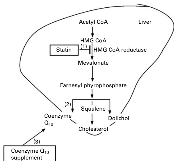
Fig. 2. Proposed mechanism by which coenzyme Q 10 supplements may support statin therapy. Statins inhibit the enzyme hydroxymethylglutaryl CoA (HMG-CoA) reductase (1) in the mevalonate pathway. The same pathway is shared by coenzyme Q 10 and as a consequence coenzyme Q 10 synthesis is inhibited (2) (112,113) . Coenzyme Q 10 supplements may raise the levels of coenzyme Q 10 (3) in plasma and platelets.
