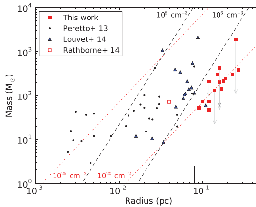
Figure 2. Solid red squares – masses assuming T_{dust} = 20 K and arrows indicate the range of mass given strong lower-mass limits estimated assuming (where possible) that T_{dust} = T_{gas} . Black points & blue triangles – high-mass proto-stellar cores in the disk (Peretto et al. 2013, Louvet et al. 2014). Open red square – star-forming core in cloud ‘a’ (ALMA, Rathborne et al. 2014). Red (dash/dot) – constant surface density, black (dashed) – constant volume density. Solid black vertical line at 0.08 pc – SMA synthesised beam.
