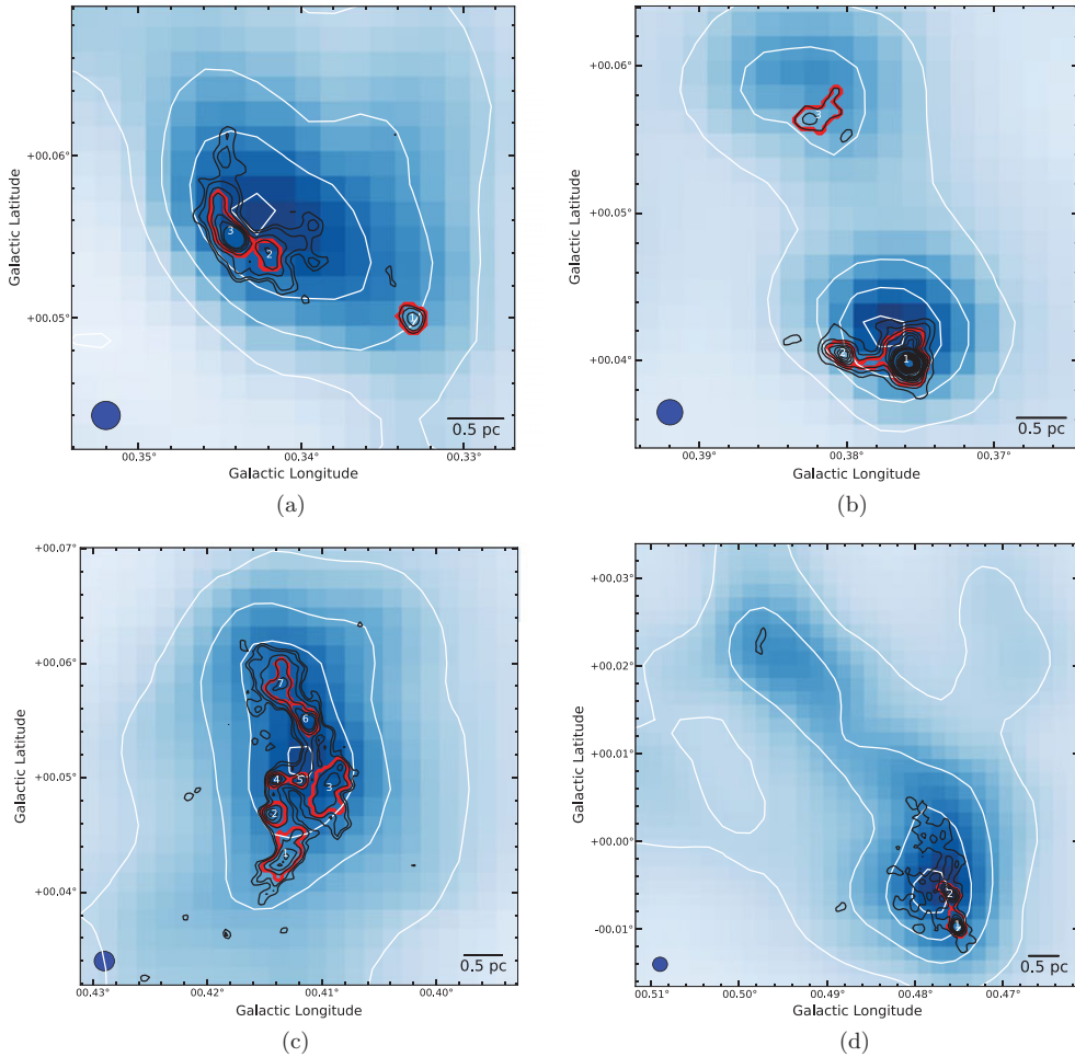
Figure 1. Top: dust ridge clouds ‘b’ (left) and ‘c’ (right). Bottom: dust ridge clouds ‘d’ (left) and ‘e/f’ (right). Background image is a Herschel column density map (Battersby et al. in prep.), shown with corresponding white contours. Black contours show the 1.3 mm continuum emission as seen with the SMA at the 5- \sigma level. Red contours highlight the cores as determined via dendrogram analysis.
