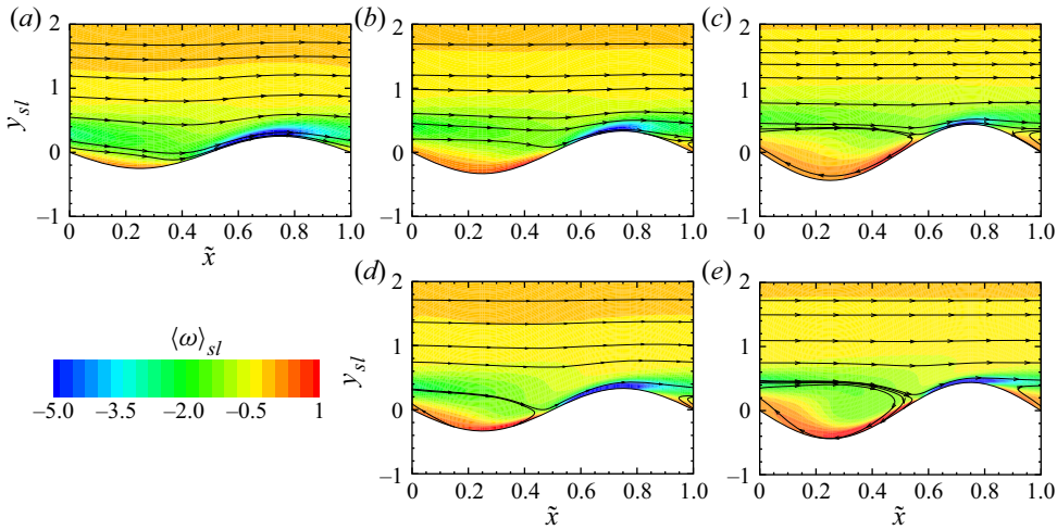
Figure 7. Contours of \langle \omega \rangle_{sl} superimposed with streamtraces of the velocity field for: (a) a^+ = 9, \lambda = \pi/8 ; (b) a^+ = 9, \lambda = \pi/16 ; (c) a^+ = 9, \lambda = \pi/32 ; (d) a^+ = 18, \lambda = \pi/8 ; and (e) a^+ = 36, \lambda = \pi/8 .
