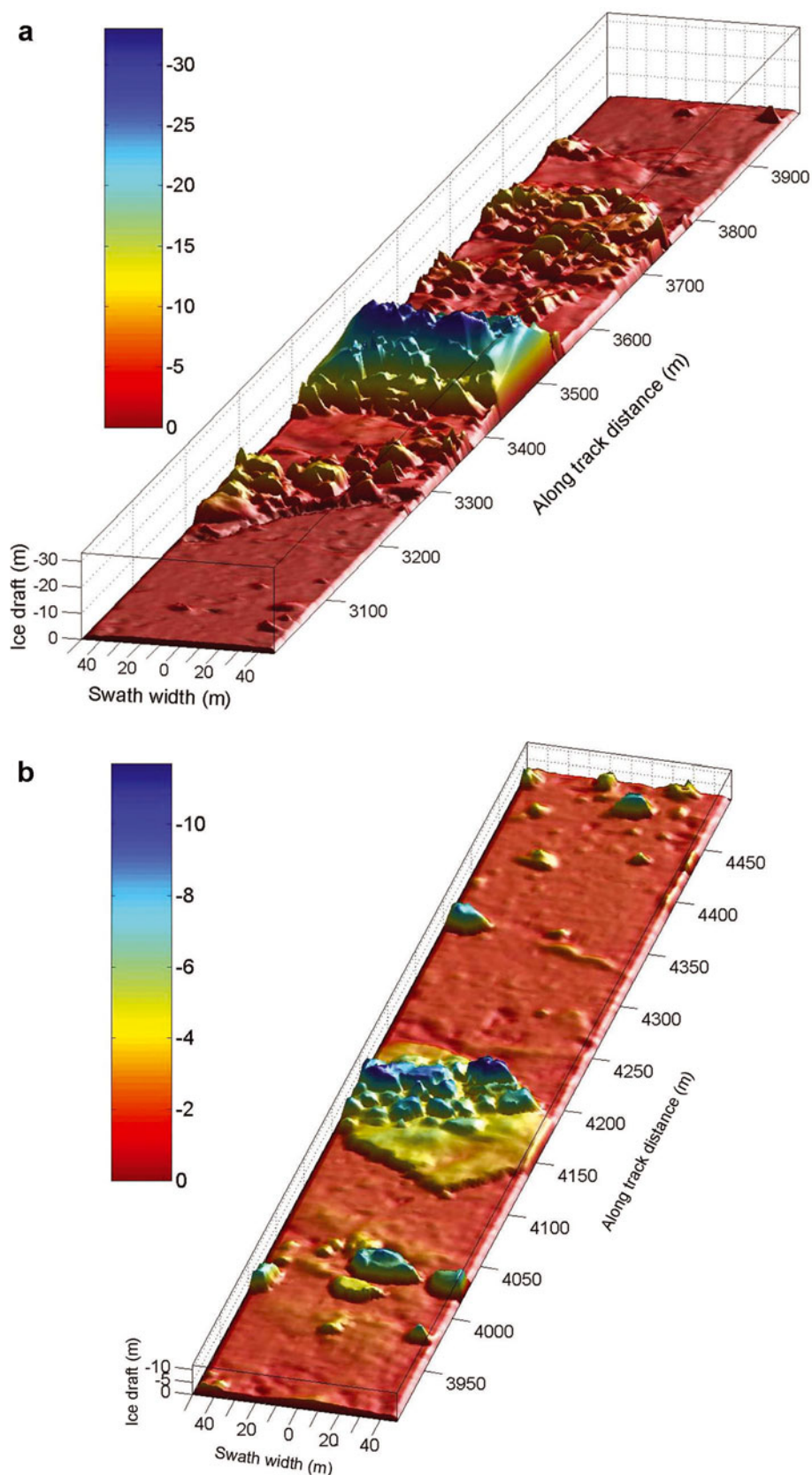
Fig. 6. Examples of EM-2000 swath-bathymetric images of the under surface of sea ice offshore of northeast Greenland. The perspective views are illuminated by a sun elevation of 20°. (a) An embedded multi-year floe with a 33 m deep sea-ice ridge. The floe is surrounded by undeformed shorefast sea ice. (b) A multi-year ridged floe of draft 3–5 m, embedded in undeformed shorefast ice of draft 1.8 m. Fast ice shows a pattern of depressions due to mirroring of surface melt pools. The floe contains a pressure ridge of maximum draft 11 m, which has partly disintegrated into individual ice blocks of diameter 5–20 m (from Wadhams and others, 2006).
