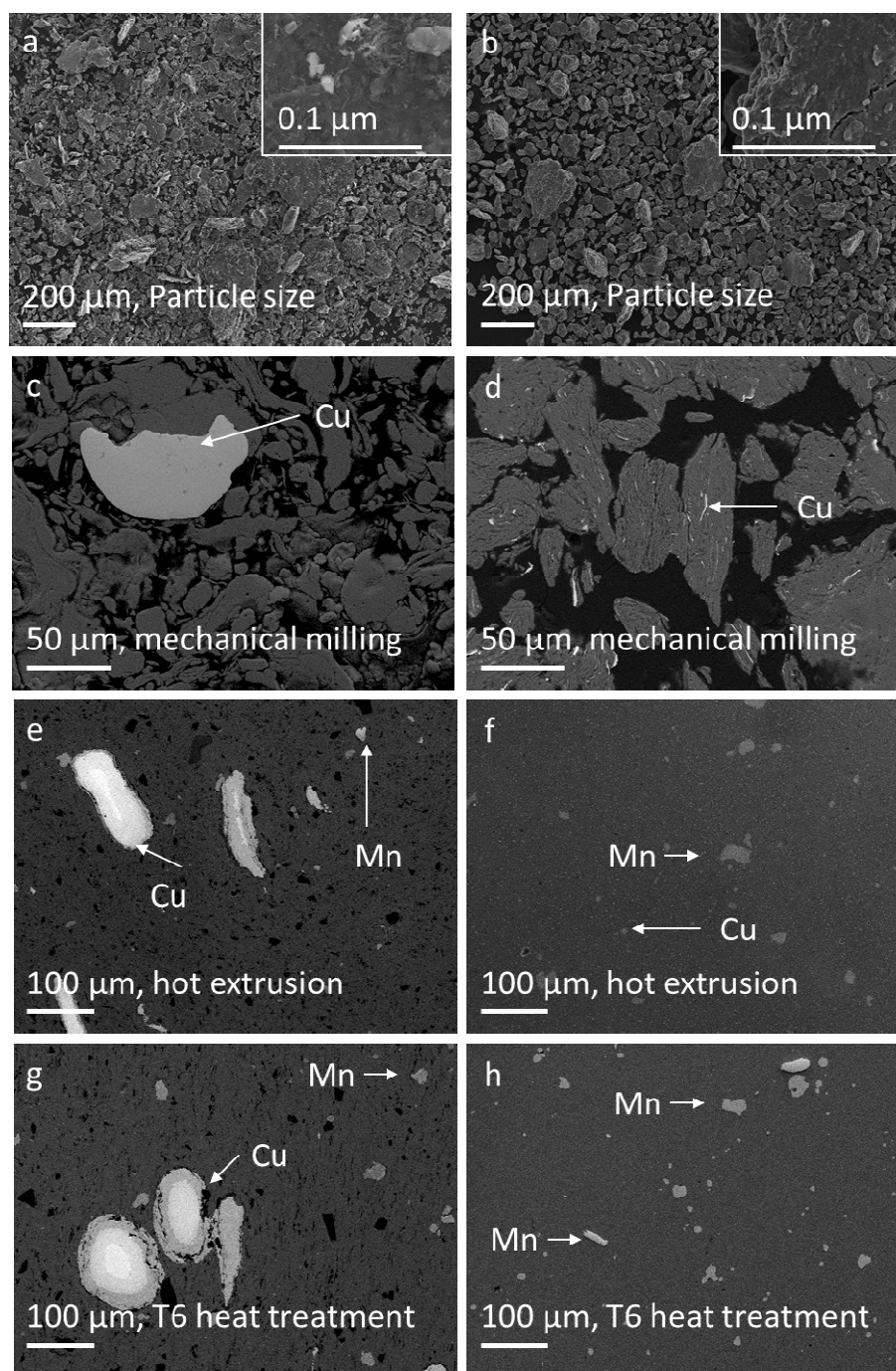
FIG.1. SEM micrographs of the Al 2024 -CNTs reinforced with 5.0 wt. % of CNTs under different processing conditions. (a, c, e and g) composites with 0.5 h of milling. (b, d, f and h) composites with 5 h of milling.
