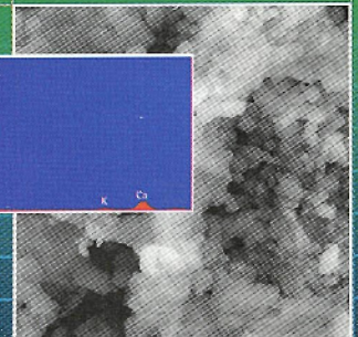
Lead oxide, uncoated, 21kV, 10,000x, chamber pressure 34 Pa, VPSE detector
