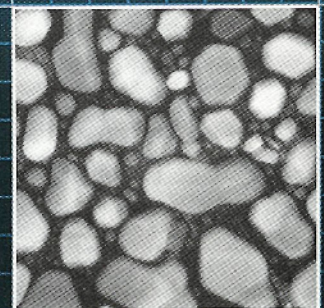
Gold on carbon, 30kV, 50,000x, chamber pressure 40 Pa, VPSE detector
