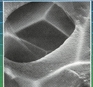
Styrofoam, uncoated, 30kV, 1,000x, chamber pressure 35 Pa, VPSE detector
