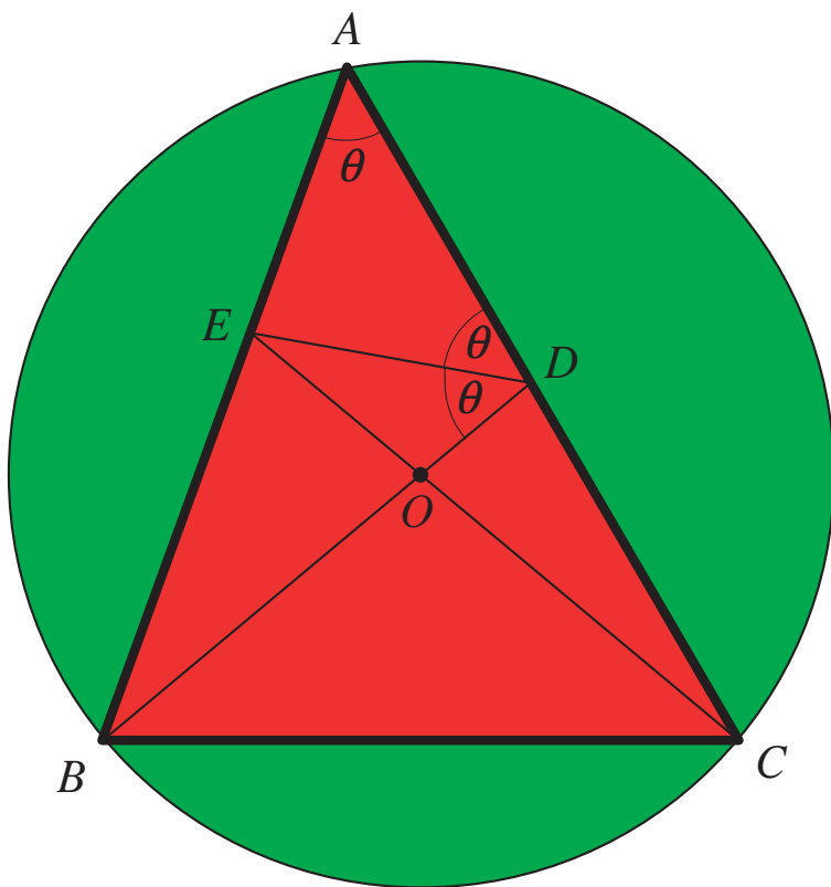
Beetham's Triangle
