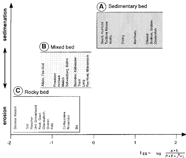
Fig. 3. Glacier-bed characteristics and I_{es} values from selected glaciers in the western Swiss Alps (modified from Haerberli, 1986).
