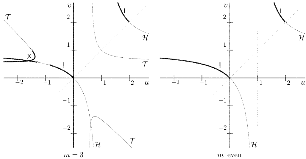
FIGURE 1. The components !, | of \mathcal{C} and, for odd m , the two beams of X , are the thick curve segments, each contained in \mathcal{H} except for the \mathcal{T} -beam of X , contained in \mathcal{T} . For m = 3 , the set \mathcal{T} consists of the isolated point (0, 0) and three disjoint real-analytic curves in \mathbb{R}^2 , diffeomorphic to \mathbb{R} . (See Remark 30.5.)
