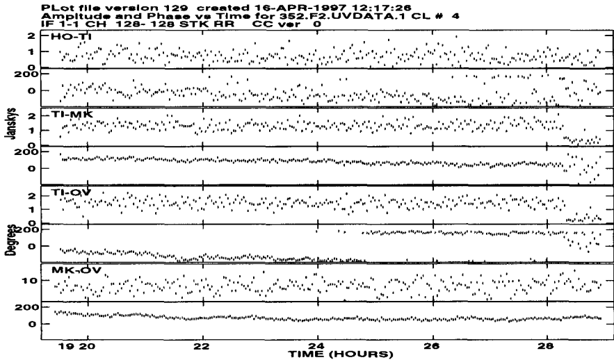
Figure 1. VLBA correlator results from the SURFSAT satellite pass on day 352, 1996. “Raw” correlator amplitude and phase are shown (no fringe-fitting), after application of the space VLBI time corrections to remove the effects of the two-way phase transfer through the SURFSAT satellite.
