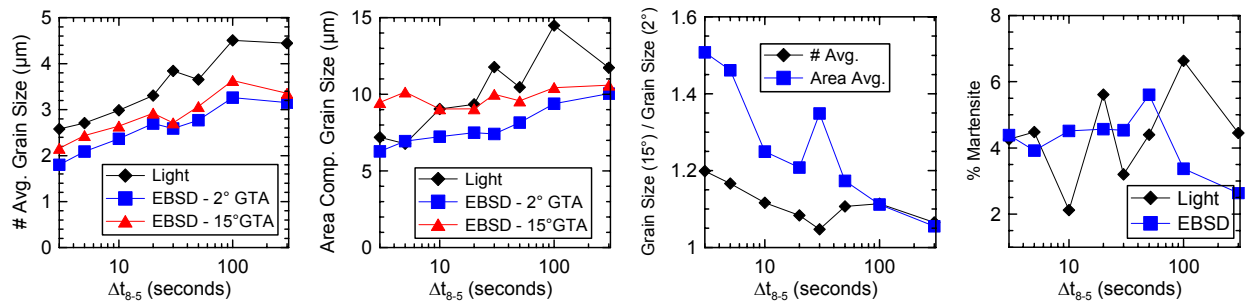
Figure 2. Grain size and martensite content as a function of \Delta t_{8-5} .
