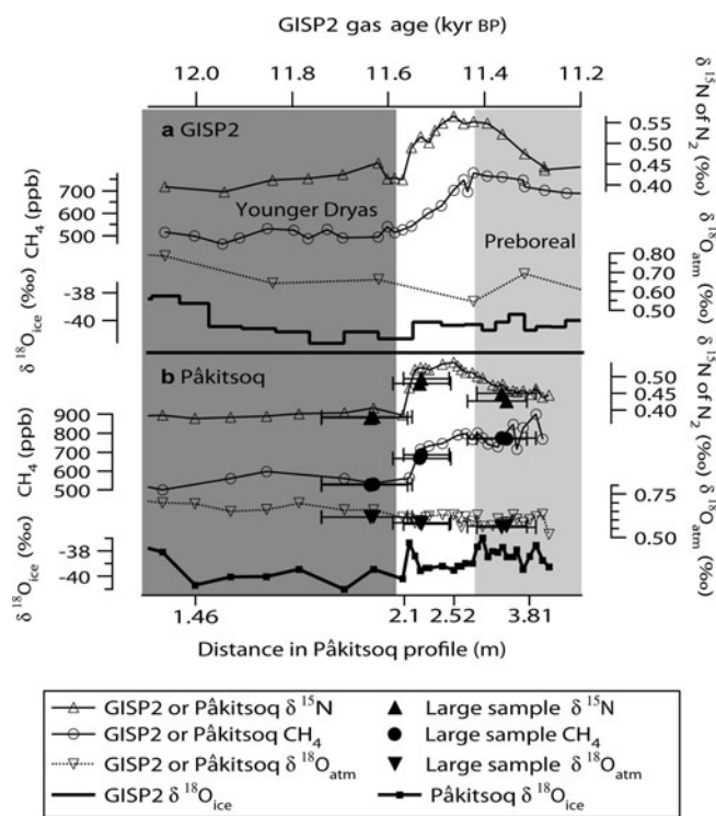
Fig. 4. Geochemical records of the YD-Preboreal transition (a) in the GISP2 ice-core record and (b) at the Pâkitsoq ice outcrop in 2004. Both records are plotted vs gas age for easy comparison. The gas age scale for Pâkitsoq was established as described in section 5, and the distances of the main age tie points in the Pâkitsoq horizontal profile are indicated. The age-distance relationship in Pâkitsoq ice is variable (Petrenko and others, 2006). For example, for the Pâkitsoq ice section shown on the plot, ice containing gases of Preboreal age is relatively less thinned. (a) GISP2 \delta^{15}\text{N} of \text{N}_2 is from Severinghaus and others (1998), [\text{CH}_4] is from Brook and others (2000) and \delta^{18}\text{O}_{\text{ice}} is from Grootes and Stuiver (1997). All GISP2 data are plotted on the gas age scale as in Schaefer and others (2006). (b) \delta^{15}\text{N} of \text{N}_2 , \delta^{18}\text{O}_{\text{atm}} and [\text{CH}_4] in the Pâkitsoq large air samples and \delta^{15}\text{N} of \text{N}_2 , \delta^{18}\text{O}_{\text{atm}} , [\text{CH}_4] and \delta^{18}\text{O}_{\text{ice}} in small ice samples taken for stratigraphic age control. The horizontal error bars on the large air samples indicate the maximum possible range of gas ages included in the samples with respect to the GISP2 gas age scale. Measurements of \delta^{15}\text{N} on the large air samples were performed simultaneously with measurements of \delta^{18}\text{O} of \text{O}_2 as described in the text. Measurements of \delta^{15}\text{N} , \delta^{18}\text{O}_{\text{atm}} , [\text{CH}_4] and \delta^{18}\text{O}_{\text{ice}} on the small ice samples were performed as described in Petrenko and others (2006). The pooled standard deviation for the small ice sample measurements was 0.009‰ for \delta^{15}\text{N} and 0.024‰ for \delta^{18}\text{O}_{\text{atm}} . The average standard deviation of the small ice sample [\text{CH}_4] measurements (includes reproducibility of repeated measurements on the same sample as well as variation in the methane blank) was 26 ppb. The age-control small ice sample set consisted of a single horizontal sample profile collected near the northern end of the sampling area (strike of the stratigraphy is approximately north-south), along with samples from the corners of ice areas cut for each large sample (not shown). Note that sample age decreases with profile distance for the YD-PB transect but increases with profile distance for the OD-Bølling transect (Fig. 5). This is due to these transects lying on opposite sides of the axis of a large-scale fold in the ice; for a more detailed discussion see Petrenko and others (2006). The Pâkitsoq deposition site is slightly warmer than Summit (with \delta^{18}\text{O}_{\text{ice}} higher by 1–2‰), with slightly thinner firn (as indicated by \sim 0.02\% lower \delta^{15}\text{N} ). This predicts a slightly lower gas-age/ice-age difference for Pâkitsoq than for GISP2. This has been taken into account when using inflection points in the Pâkitsoq \delta^{18}\text{O}_{\text{ice}} record to establish gas-age tie points.
