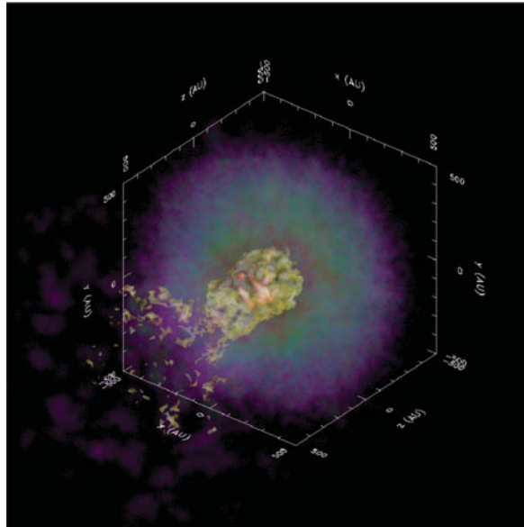
Figure 1. 3D rendering of an asymmetric core-collapse supernova explosion model from Hungerford et al. (2005), one year after the shock launch. The top-hat distribution of the imposed velocity asymmetry allows a significant portion of the cone material to expand without drag from fluid shear forces, resulting in the large splash of material at the outer ejecta. This and similar hydrodynamical models will be coupled with dust formation models and used as input for SKIRT radiative transfer simulations.
