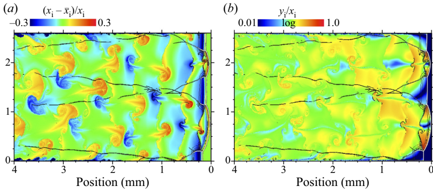
Figure 10. Diluted 2H 2 –O 2 –7Ar mixture. The 2-D instantaneous Lagrangian flow fields, superimposed with Schlieren density in diluted 2H 2 –O 2 –7Ar mixture. (a) Normalized fluctuations of the longitudinal distances (x_i - \bar{x}_i)/x_i . (b) Normalized transverse distance y_i/x_i .
