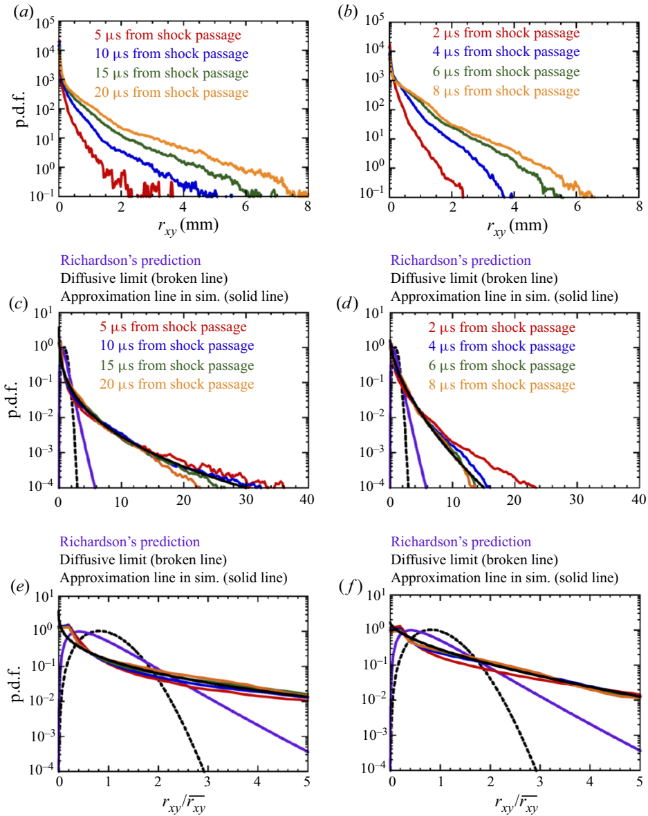
Figure 22. (a,c,e) The 2\text{H}_2\text{-O}_2\text{-7Ar} mixture; (b,d,f) 2\text{H}_2\text{-O}_2 mixture. (a,b) The p.d.f. for relative dispersion r_{xy} ; (c,d) p.d.f. for r_{xy}/\bar{r}_{xy} ; (e,f) enlarged view of p.d.f. for r_{xy}/\bar{r}_{xy} .
