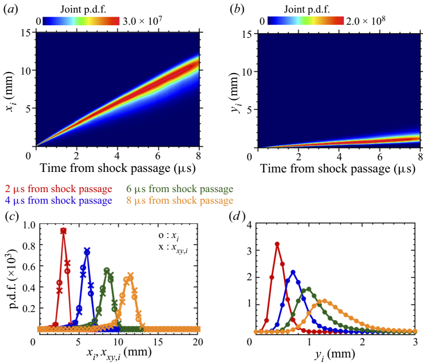
Figure 9. The 2H 2 –O 2 mixture. Joint p.d.f. between (a) times from shock passage and longitudinal distances x_i , (b) times from shock passage and transverse distances y_i . The p.d.f. at different instants for (c) longitudinal distances x_i and distances x_{xy,i} , (d) transverse distances y_i .
