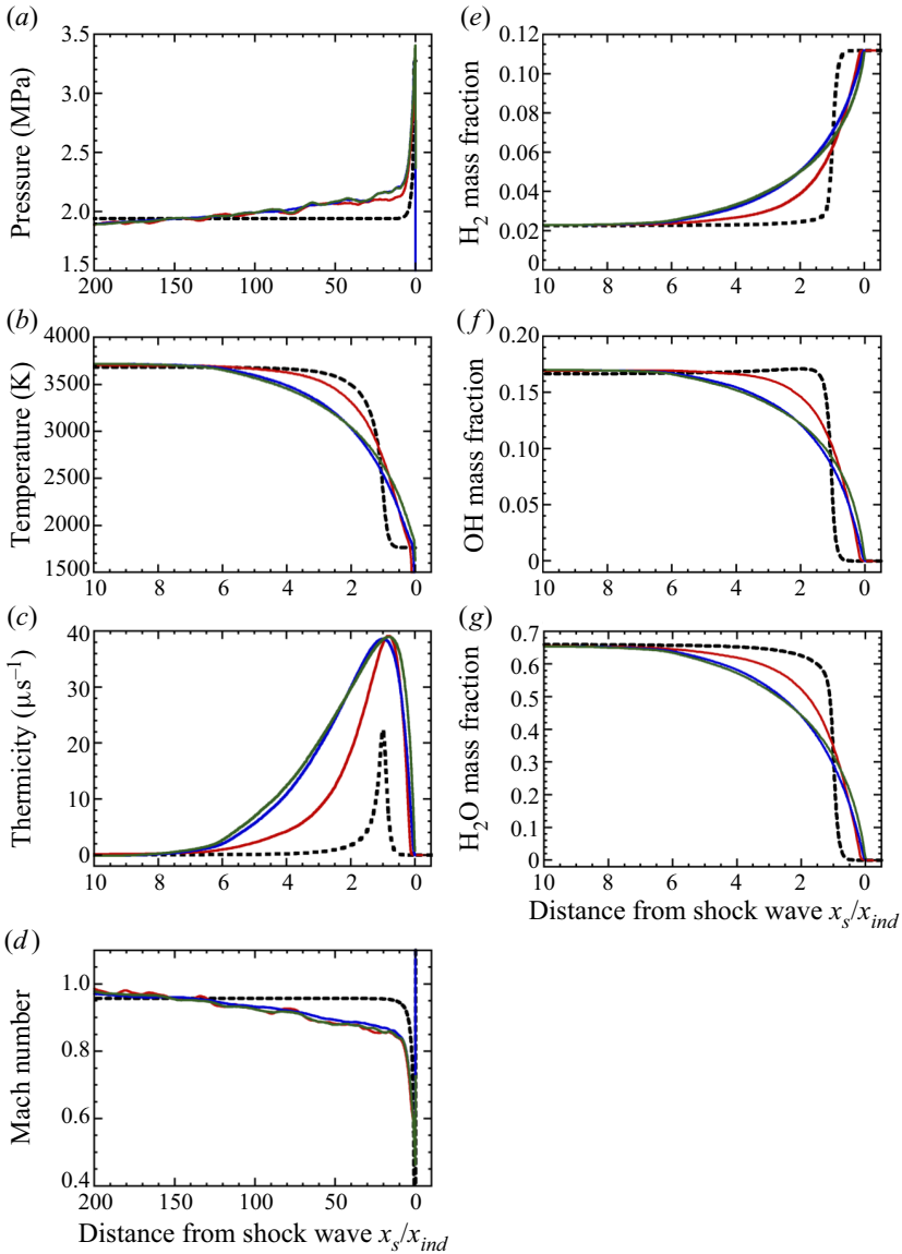
Figure 29. Favre average 1-D profiles in 2\text{H}_2\text{-O}_2 mixture for (a) pressure, (b) temperature, (c) thermicity, (d) Mach number, (e) \text{H}_2 mass fraction, (f) OH mass fraction, and (g) \text{H}_2\text{O} mass fraction.
