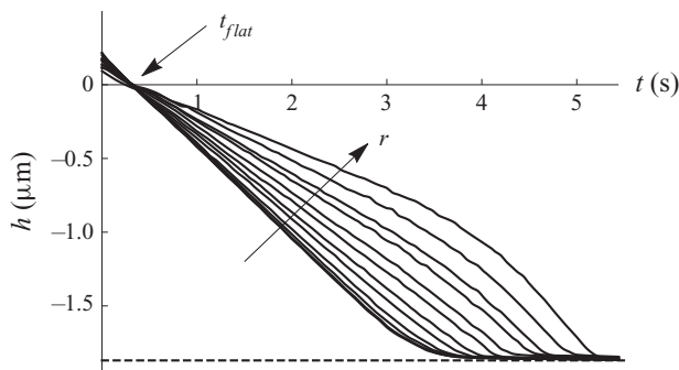
Figure 15. Experimental results for the free-surface profile h of a droplet as functions of t for r = 0, 4.29, 8.57, 12.86, 17.68, 20.90, 26.79, 30.01, 32.15, 34.83 and 38.04 for the 50\ \mu\text{m} well. The arrow indicates the direction of increasing r . The dashed line corresponds to the depth H_0 = 1.87\ \mu\text{m} of the well.
