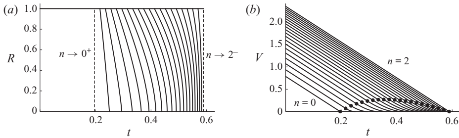
Figure 3. Plots of (a) the radius R of the receding contact line given by (4.14), and (b) the volume V of the droplet given by (3.21d) for 0 \leq t \leq t_{touchdown} and by (4.15) for t_{touchdown} < t \leq t_{lifetime} as functions of t for n = 0, 1/10, 1/5, \dots, 2 in the case H_0 = 1 . The vertical dashed lines in (a) correspond to the limits n \rightarrow 0^+ and n \rightarrow 2^- , and the dots in (b) correspond to touchdown (at the lip of the well) at t = t_{touchdown} = \pi(1 + nH_0)/16 .
