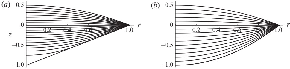
Figure 2. Evolution of the free-surface profile h given by (3.21a) for 0 \leq t \leq t_{touchdown} and by (4.2) for t_{touchdown} < t \leq t_{lifetime} for (a) a conical well with n = 1 and H_0 = 1 , and (b) a paraboloidal well with n = 2 and H_0 = 1 . In (a) the curves are drawn at intervals of t_{touchdown}/16 = \pi/128 \simeq 0.0245 , and the lifetime is t_{lifetime} = 5\pi/32 \simeq 0.4909 , while in (b) the curves are drawn at intervals of t_{touchdown}/15 = \pi/80 \simeq 0.0393 , and the lifetime is t_{lifetime} = t_{touchdown} = 3\pi/16 \simeq 0.5890 .
