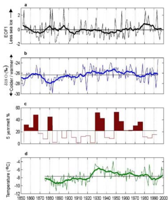
Fig. 6. (a) Time series of EOF1 for the period 1852–1997. The bold line is an 11 year running mean to highlight decadal variability. (b) Same as (a) but for \delta^{18}\text{O} values. (c) Five-year averages of melt percentages from the D99 core. (d) Measured SAT at Upernavik for the period 1875–1999, with 11 year running mean bold line. The black horizontal lines on each graph represent the mean of the series.
