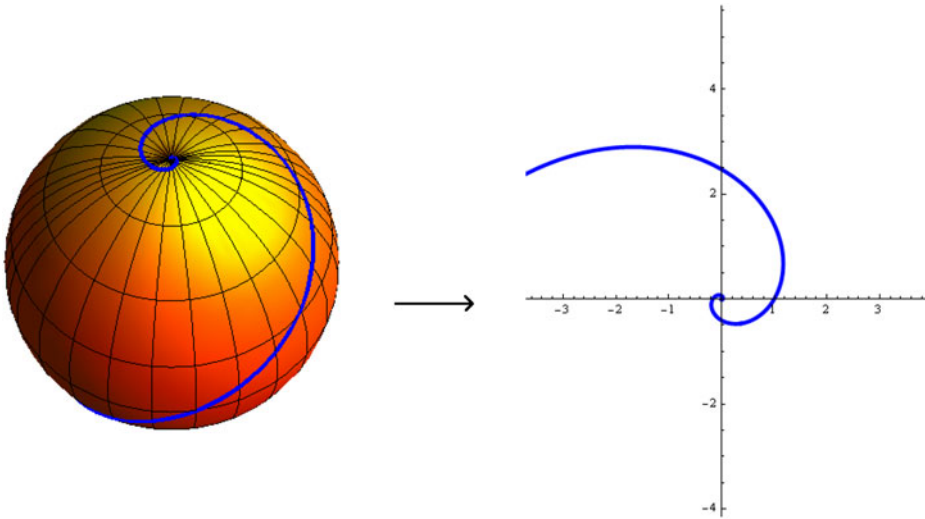
Figure 1. Stereographic projection of a loxodrome on a sphere (Babaarslan and Munteanu, 2013).
