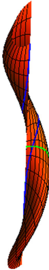
Figure 3. The helicoidal surface; loxodrome (blue), meridian (green).
