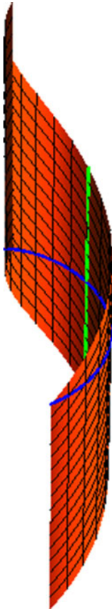
Figure 2. The helicoidal surface; loxodrome (blue), meridian (green).
