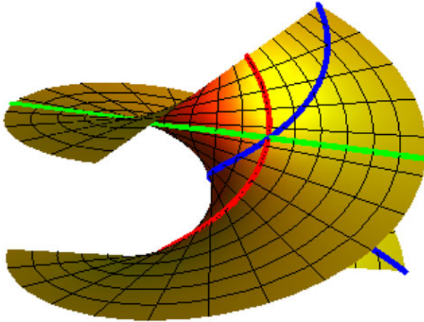
Figure 4. The right helicoidal surface (helicoid); loxodrome (blue), meridian (green), parallel (red).
