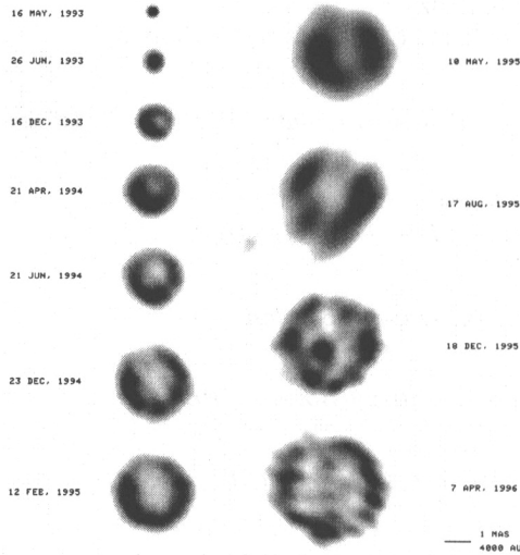
Figure 1. Images of SN 1993J at 8.4 GHz, phase-referenced to the core of M81. The relative position of the 10 May 1995 image is arbitrary. The CLEAN/MEM models were restored using a Gaussian beam with a typical width of 0.6 mas. The total flux densities range from \sim 90 to \sim 20 mJy, with peak intensities between \sim 90 to \sim 1 mJy/beam. The rms background noise is \sim 0.05 mJy/beam.
