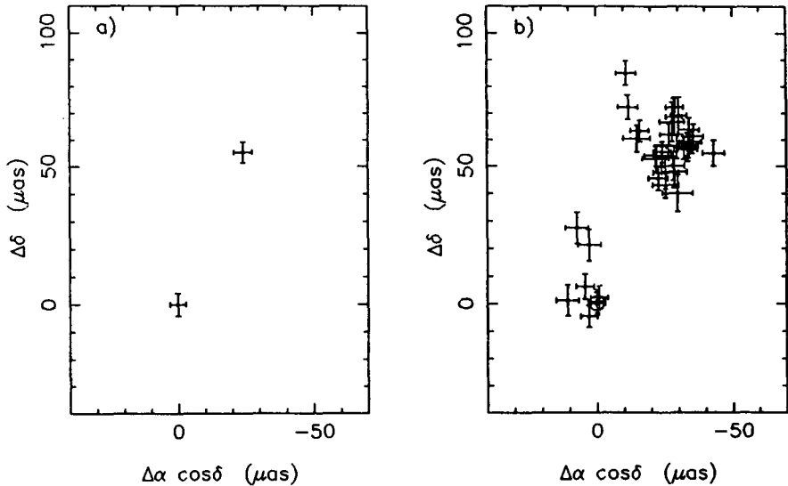
Figure 1. Estimates of the offsets of the position at \lambda=3.6\text{cm} of the core of quasar 1038+528 A, relative to 1038+528 B at epochs 1981.2 and 1983.4 (with 1981.2 offsets subtracted): (1a) our best estimate, corresponding to Table I; (1b) summary of all results from the numerical experiments described in the text.
