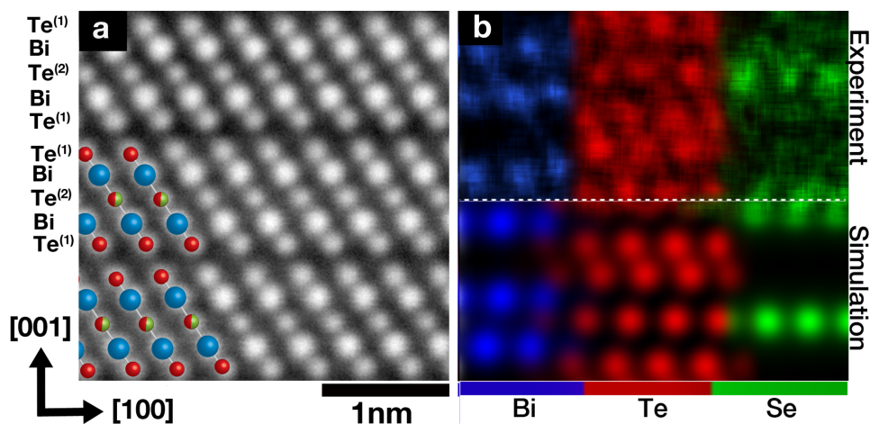
Figure 2. (a) RevSTEM image series of the nanostructured \text{Bi}_2\text{Te}_{2.7}\text{Se}_{0.3} with a schematic of the structure overlaid. (b) Experimental and simulated atomic resolution EDS showing segregation of Se to the Te(2) position.
