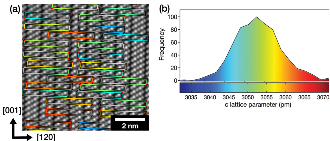
Figure 1. (a) RevSTEM image series of pure \text{Bi}_2\text{Te}_3 with boxes representing individual measured unit cells. (b) Histogram of the measured lattice parameters with the same color scale used for the box color in (a).
