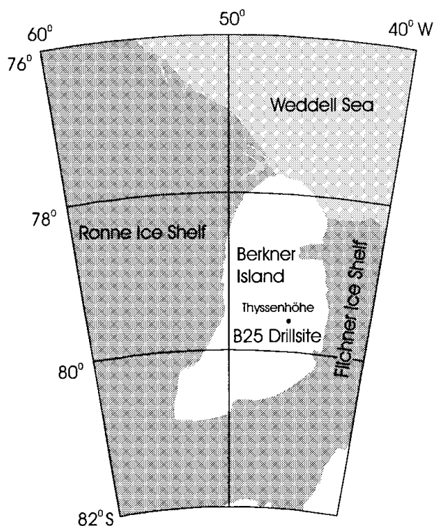
Fig. 1. Map of Berkner Island and surrounds, and drill location.
