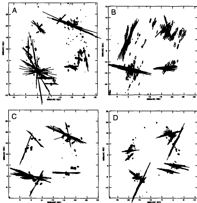
Figure 1. 4 images of the total intensity and linearly polarized electric vectors of the 43 GHz SiO maser emission from U Her. The images show the emission integrated over the velocity range of the maser: a) June 1995; b) Dec 1995; c) Feb 1995; d) Apr 1995.
