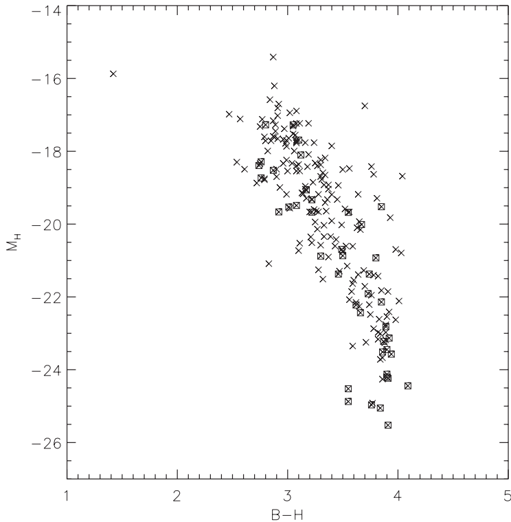
Figure 1. Optical/IR CMD for the Virgo ETGs with accurate photometry. The dusty ones (squares) are not bluer, i.e. not more star-forming, than the other galaxies (crosses).
