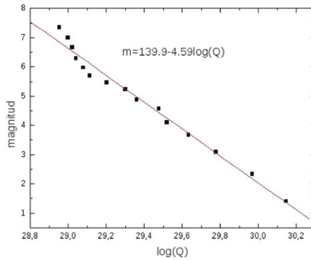
Figure 2. Calibration curve of the light curve, showing the equation of the magnitude as a function of the logarithm of the sublimation rate for comet C/1996 B2 Hyakutake, adjusted by least squares.
