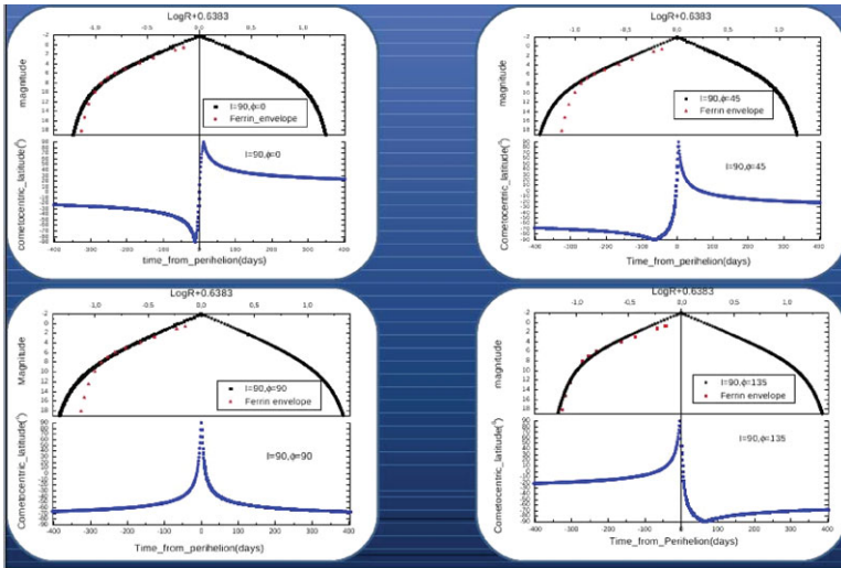
Figure 3. Seculars light curves calculate for the Hyakutake Comet considering I = 90^\circ and varying the longitude of the orbital pole.
