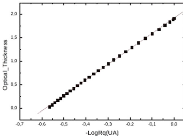
Figure 5. Optical thickness of the coma vs heliocentric distance.
