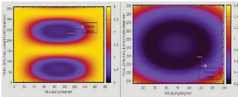
Figure 4. Contorn map made for our model for comet C/1996 B2 Hyakutake. The plot show the obliquity, I , versus the pole orbital longitude, \phi . In this plot see the standard deviation for each of the orientations of the axis of rotation with a color profile of one degree.
