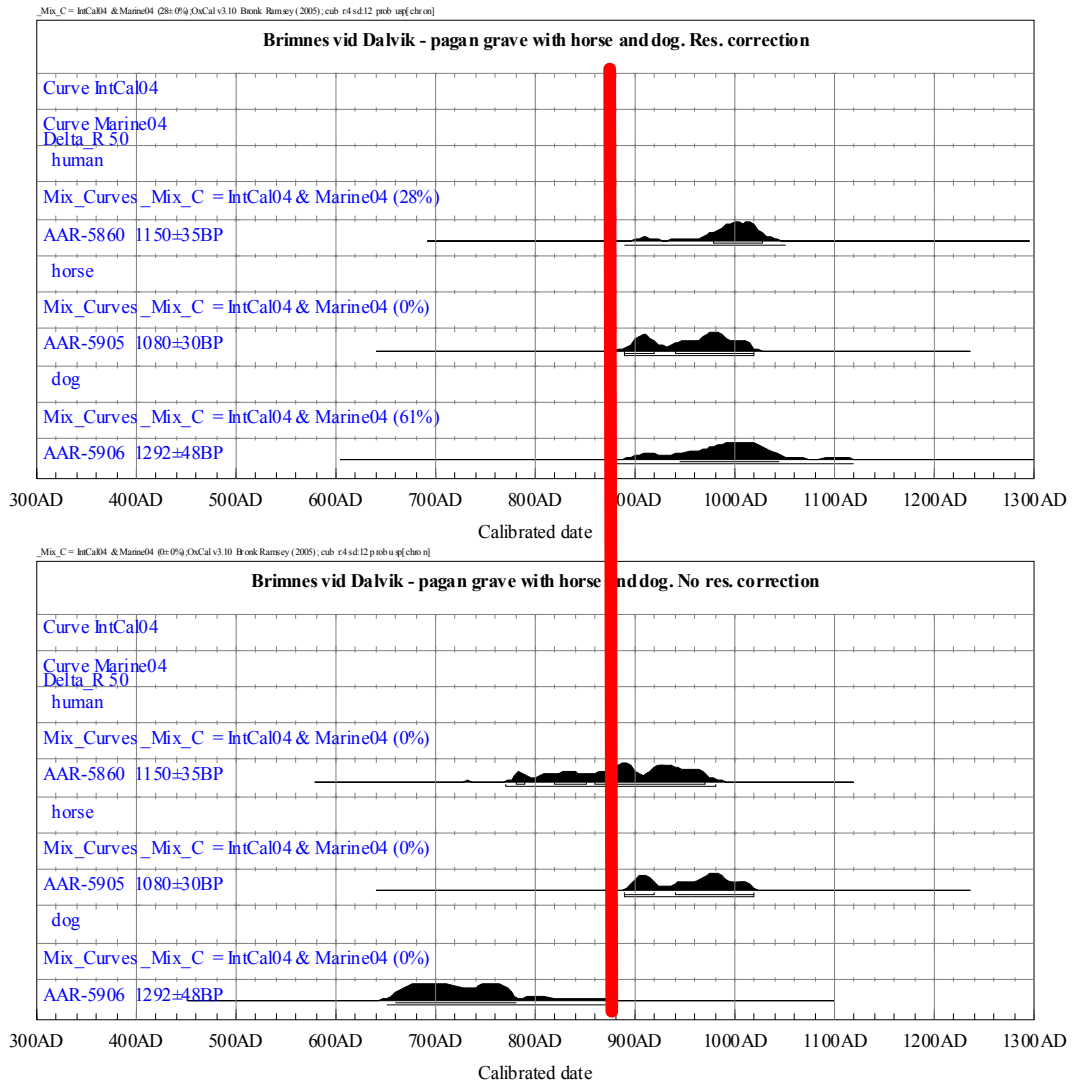
Figure 4 Reservoir age corrections were checked by comparing a) (above) 14 C dates of a horse (100% terrestrial), a dog (highly marine), and a human (mixed diet) from the same pagan burial in Brimnes, N Iceland, and b) (following page) by comparing 14 C dates of 3 human skeletons and a dog from the same burial close to Keldudalur in N Iceland. When the 14 C age is calibrated with correction for the marine reservoir effect (based on the \delta^{13}C measurements), the 3 14 C age determinations from Brimnes become identical. If no reservoir correction is applied, the dog appears considerably older than his master, and its age is inconsistent with the time of Norse settlement of Iceland around AD 874, indicated by the vertical bar. This is also the case for the Keldudalur pagan gravesite where after our correction procedure, all the dates are consistent both with the settlement time of Iceland AD 874 and with Christianity being introduced around AD 1000.
